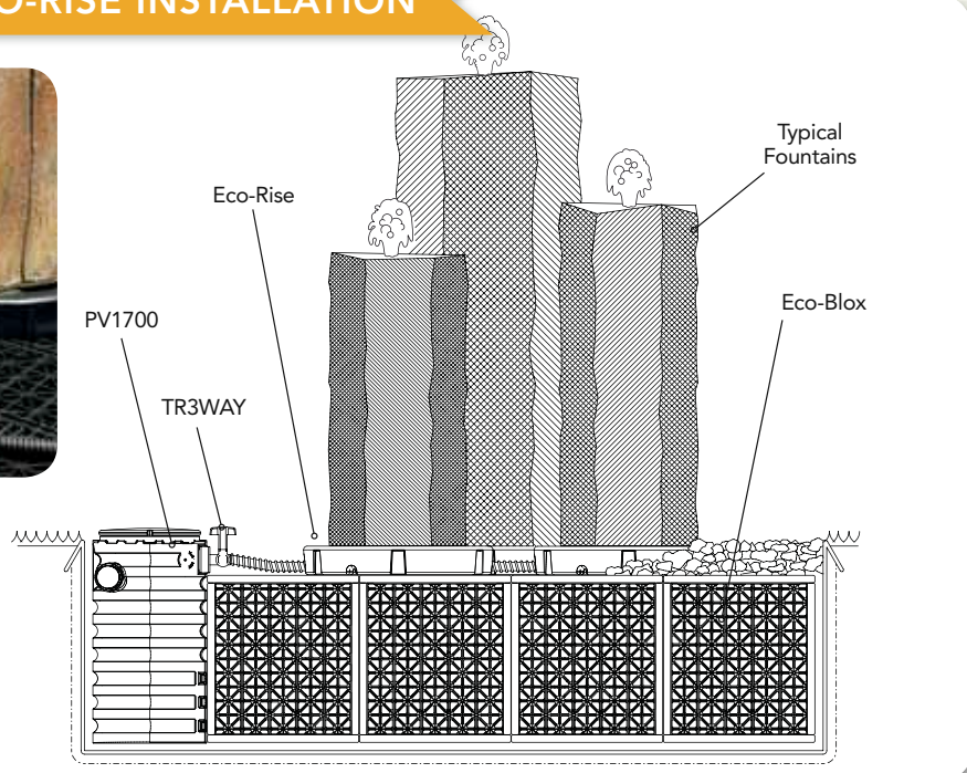
PV1700 Pump Vault shown with 3-Way Diverter installed for use with the Eco-Rise and Eco-Blox. Add a second pump and a second 3-Way Diverter to control up to six water features from a single PV1700 Vault.
